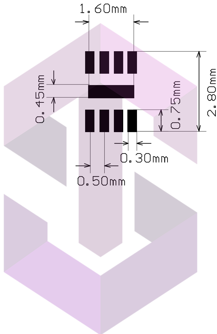
Figure 30. DFN8 2 x 2 recommended footprint
