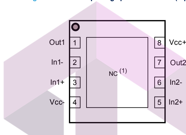
Figure 3. DFN8 2x2 package pin connections (top view)
