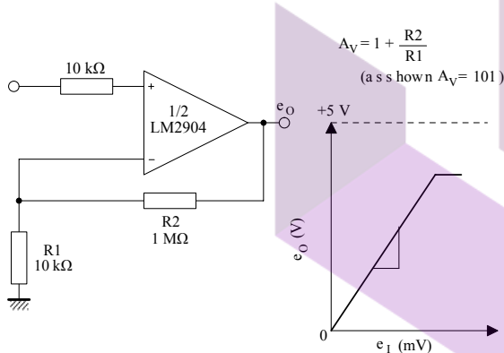
Figure 23. Non-inverting DC gain
